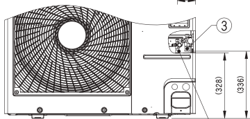
Piping connection port
